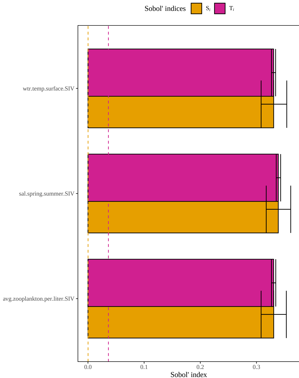
Figure 4. Results of a sensitivity analysis for the alewifeJuv model based on an arithmetic mean structure. Dashed lines represent baseline numerical approximation error for S_i and T_i ( i.e. , dummy variables).
