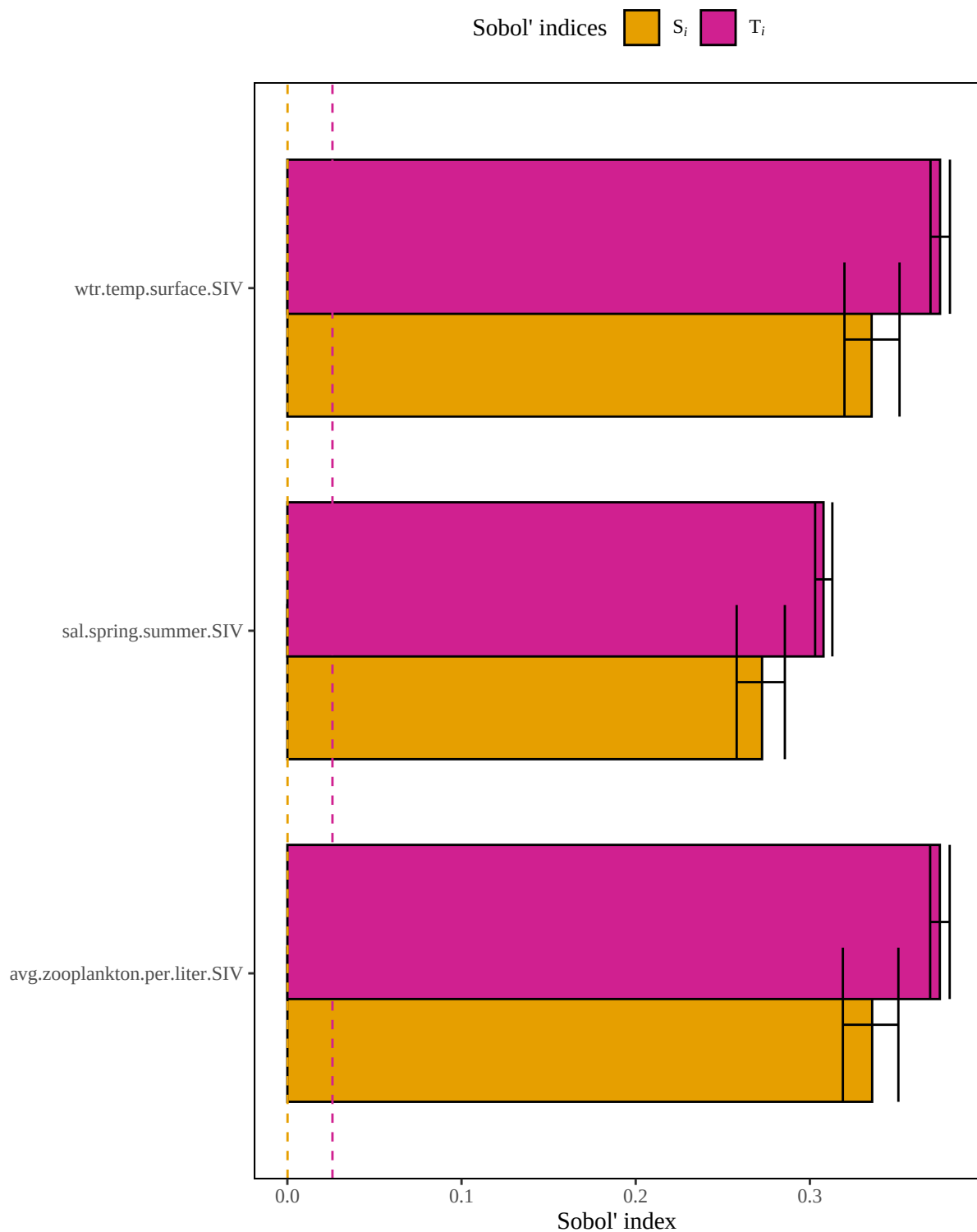
Figure 5. Results of a sensitivity analysis for the alewifeJuv model based on a geometric mean structure. Dashed lines represent baseline numerical approximation error for S_i and T_i ( i.e. , dummy variables).
